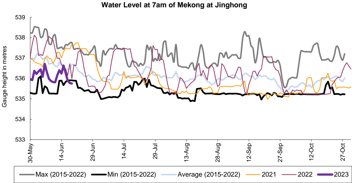
Figure 7. Water level at the Jinghong hydrological station up to 19 June 2023.
